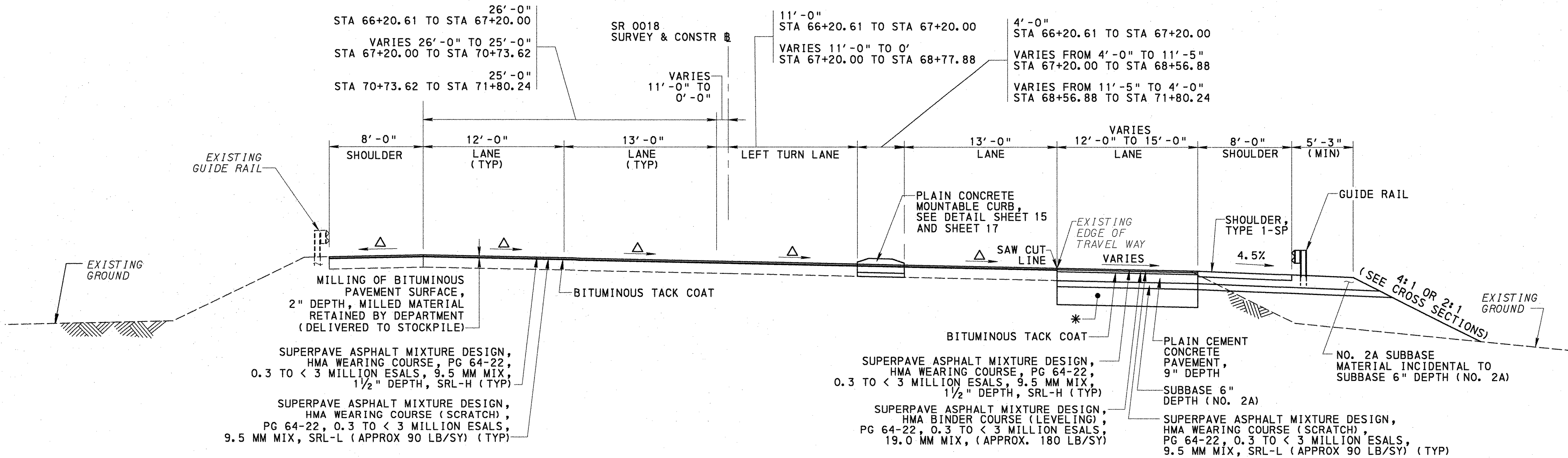
TYPICAL SUPERELEVATED SECTION SR 0018 STA 66+20.61 TO STA 71+80.24 NOT TO SCALE
