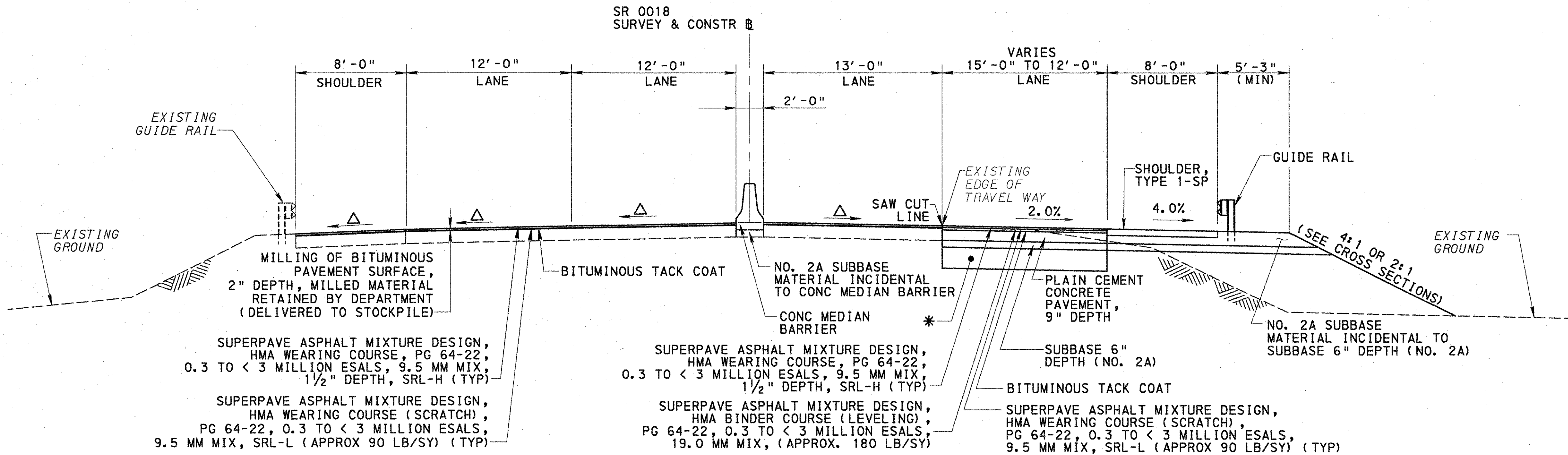
TYPICAL TANGENT SECTION SR 0018 STA 71+80.24 TO STA 73+00.00 NOT TO SCALE
